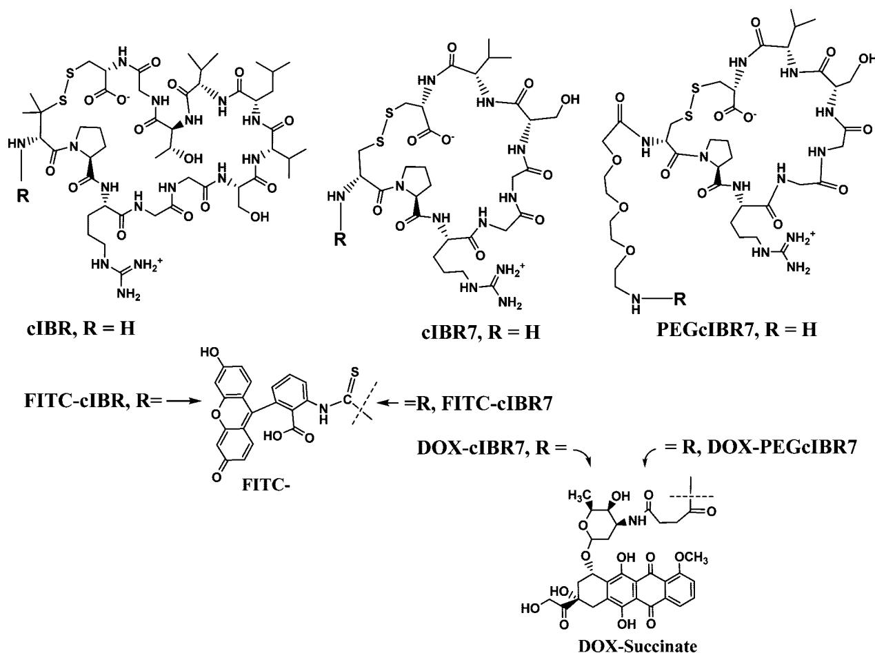
Figure 1. The chemical structures of cIBR peptide (cyclo(1,12)PenPRGGSVLVTGC) and its derivatives cIBR7 (cyclo(1,8)CPRGGSVC) and PEGcIBR7 (PEG-cyclo(1,8)CPRGGSVC). These peptides were conjugated to the carboxylic acid of DOX-succinate from their free N-terminus. cIBR7 peptide was synthesized by removing the LVTG sequence from the C-terminal of cIBR peptide. Pen1 in cIBR was replaced by Cys1 in cIBR7. PEGcIBR7 peptide was synthesized by conjugating 11-amino-3,6,9-trioxaundecanoic acid to the N-terminal of the cIBR7 peptide.
